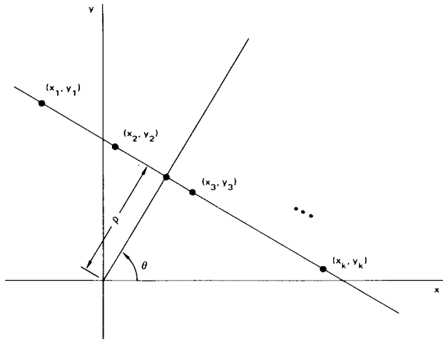
Fig. 2. Projection of colinear points onto a line.
